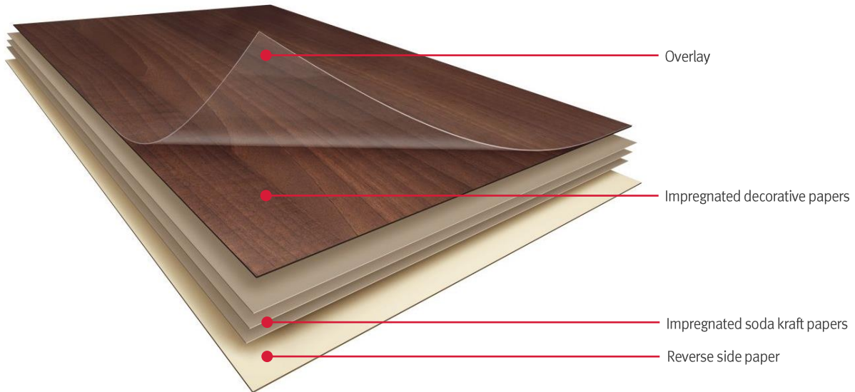
Laminate composition, showing EGGER Laminate as an example
